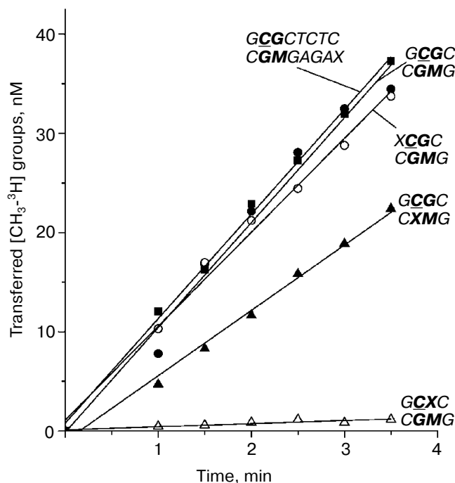
Fig. 5. Methylation of DNA duplexes by M.SssI. C_{\text{DNA}} , 0.5 \mu\text{M} ; C_{\text{M.SssI}} , 20 nM; C_{[\text{CH}_3\text{-}^3\text{H}]\text{AdoMet}} , 1.2 \mu\text{M} . Designations are as in Fig. 1.
